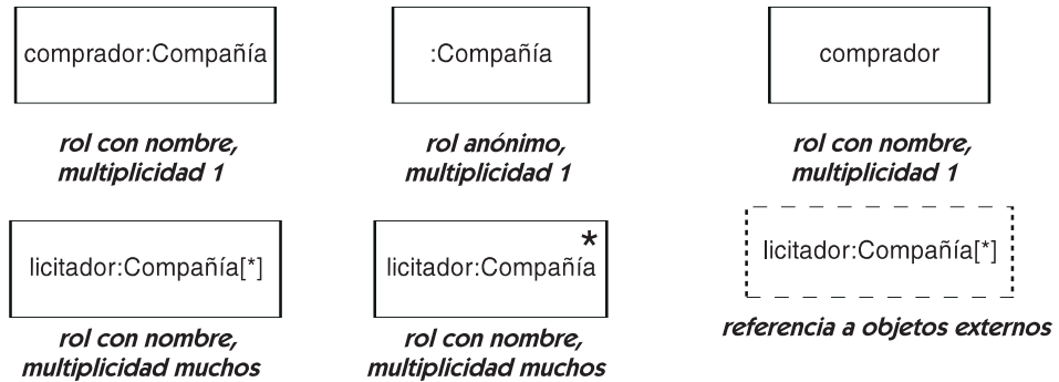
Figura 14.59 Roles o partes
